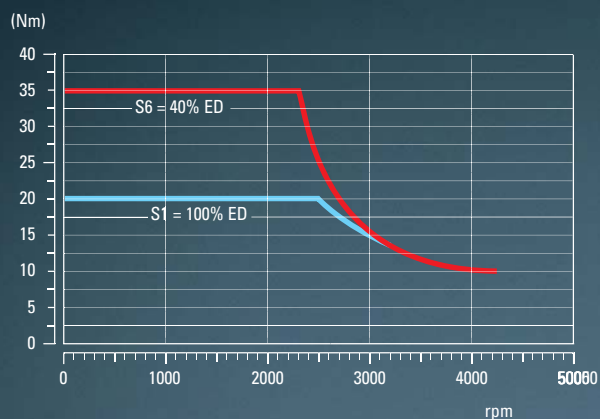
EMCOMAT 14S/14D
