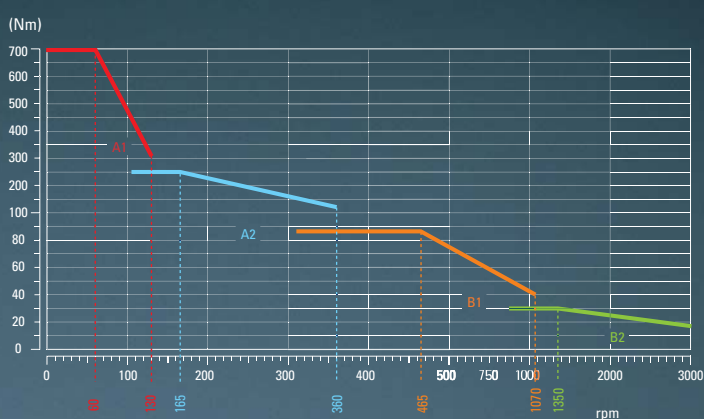
EMCOMAT 17S/17D/20D
